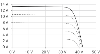
UP-Kennlinie Bsp. 430 Wp
