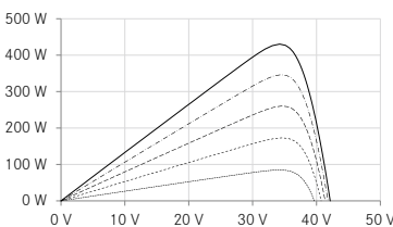
UP-Kennlinie Bsp. 430 Wp
